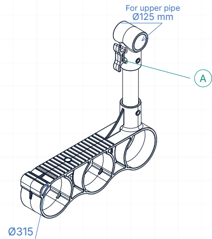
03 ISOMETRIC VIEW
