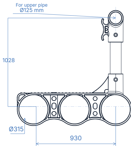
01 FRONT VIEW
