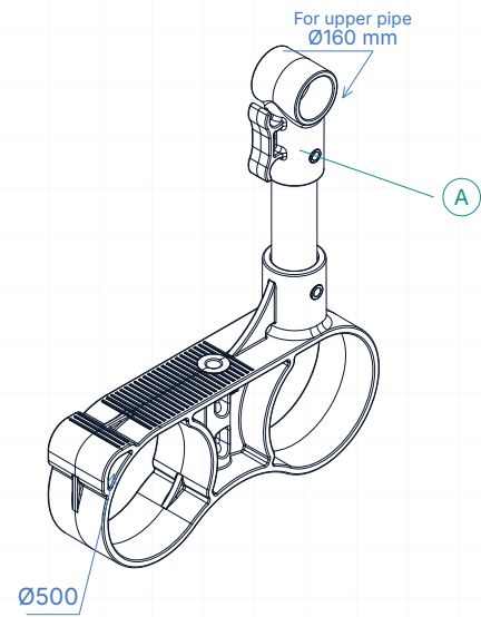
03 ISOMETRIC VIEW
