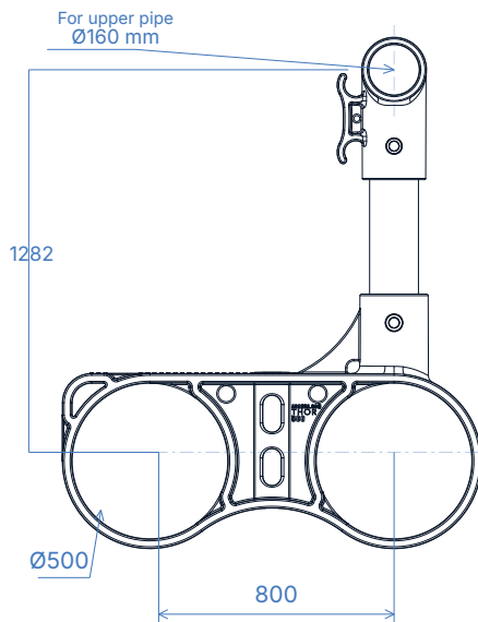
01 FRONT VIEW
