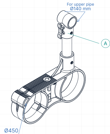
03 ISOMETRIC VIEW
