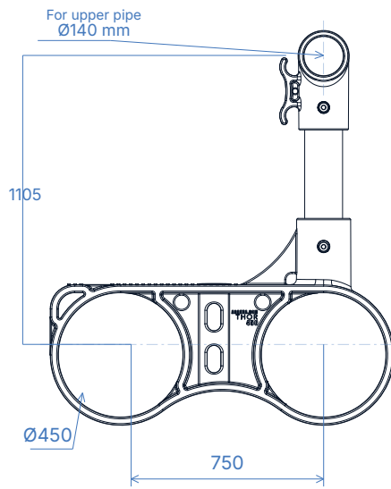
01 FRONT VIEW
