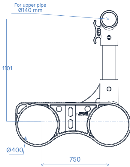
01 FRONT VIEW
