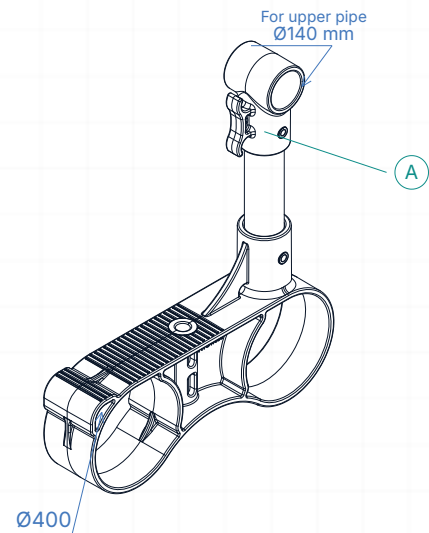
03 ISOMETRIC VIEW
