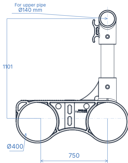
01 FRONT VIEW
