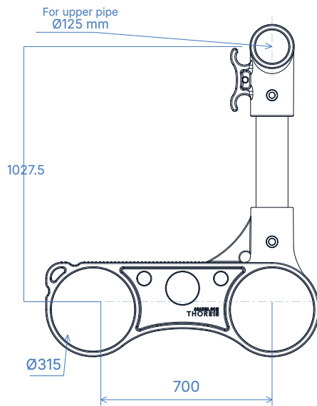
01 FRONT VIEW
