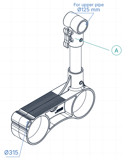
03 ISOMETRIC VIEW
