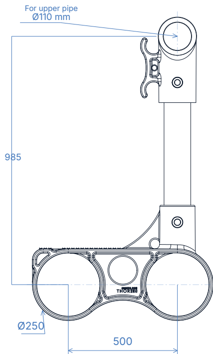
01 FRONT VIEW
