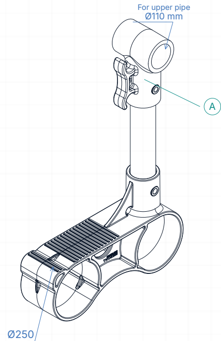
03 ISOMETRIC VIEW
